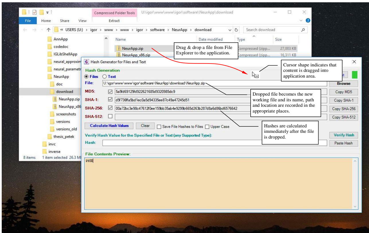
Figure 10: Drag & drop a file from the File Explorer on Windows. Files can be dragged from numerous applications that support drag & drop for files, including your desktop, file dialog boxes, and a number of third party file explorer applications available for a particular operating system (see e.g. Figure 14 for example on Linux).
