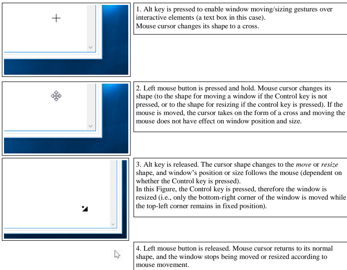
Figure 11: Stages of moving / resizing application window by using customized gestures.
