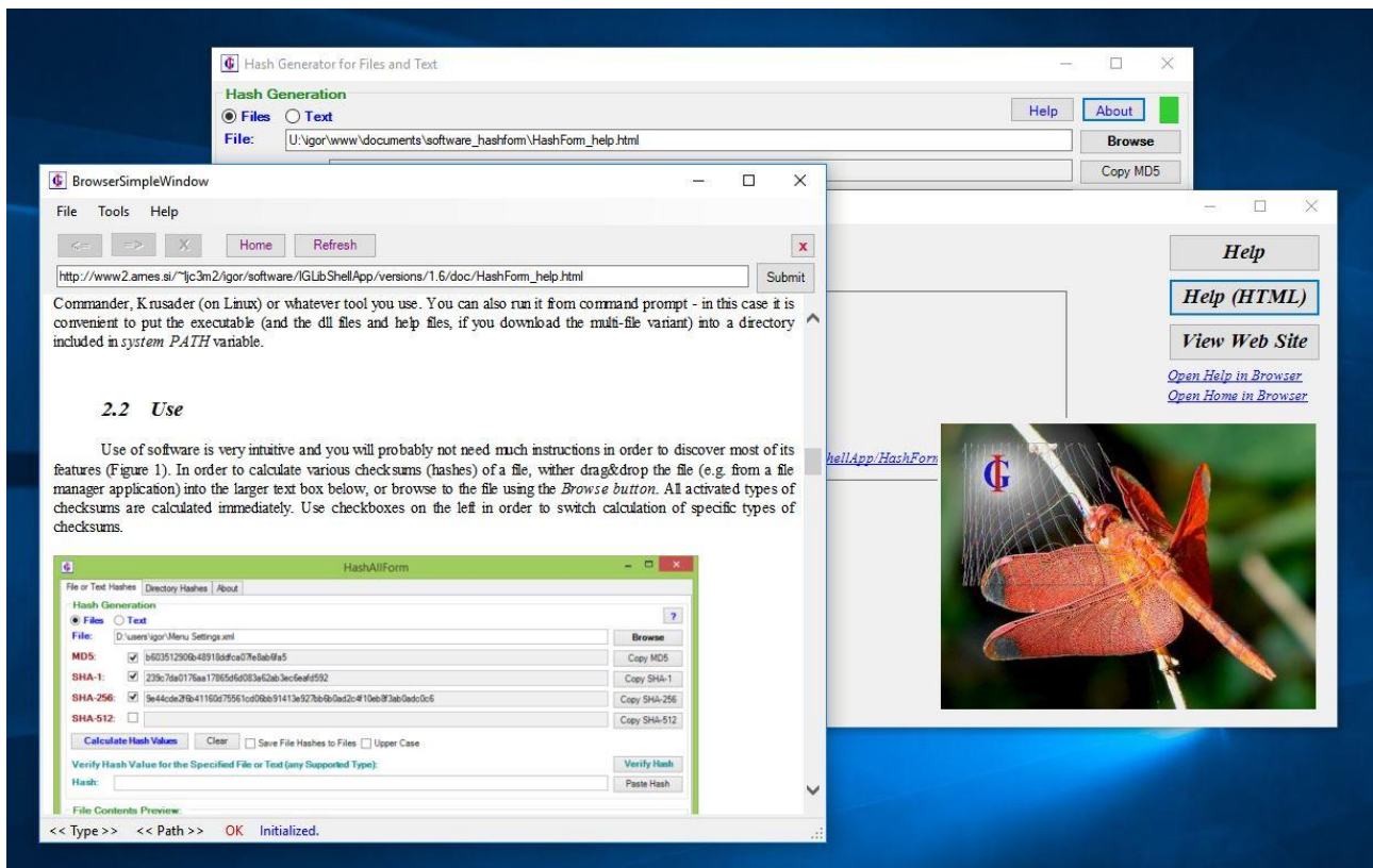
Figure 13: Information about the software can be accessed by clicking the “About” button. This opens a box with some basic information such as software version. From there, you can open documentation or home page either in a built-in browser or in system’s web browser or PDF viewer. Clicking the “Help” button in the main application window opens the user manual directly.
